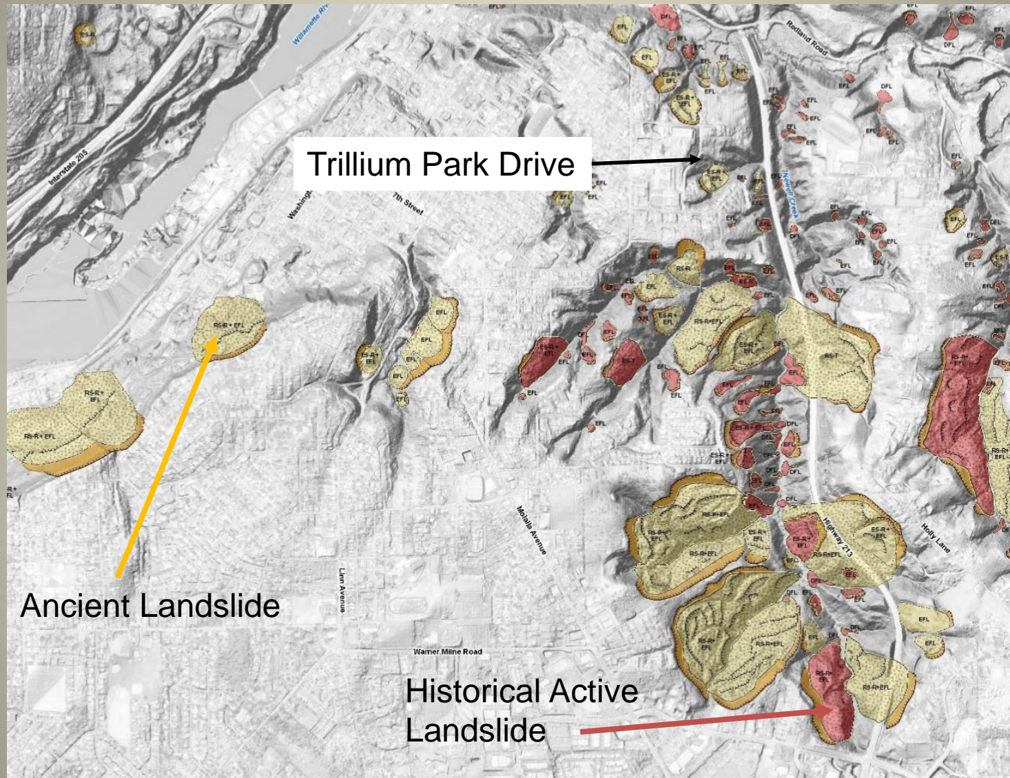
Landslide Inventory map of the Northwest Quarter of the Oregon City Quadrangle, IMS-26
